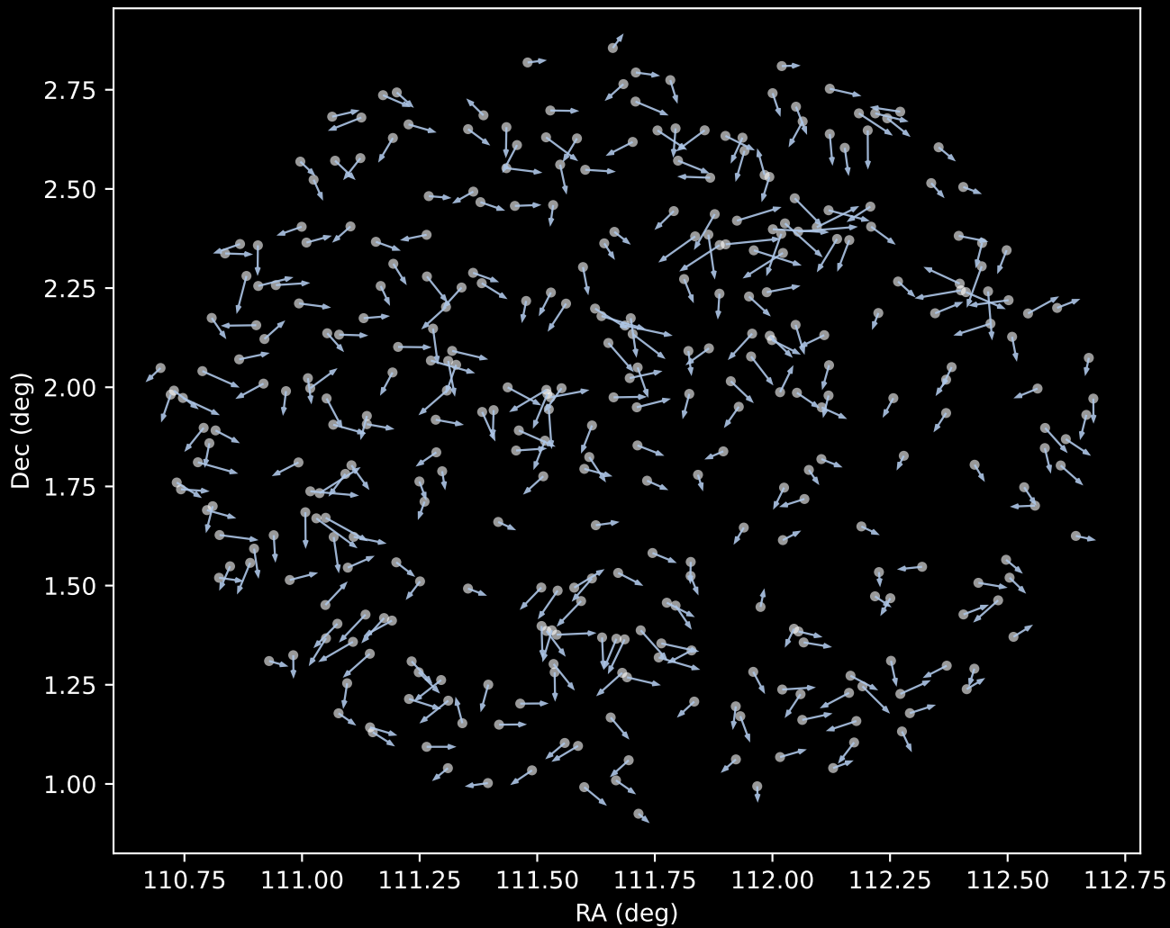
GALAH DR4 Cluster 1 Proper Motion Vectors (n=352)
