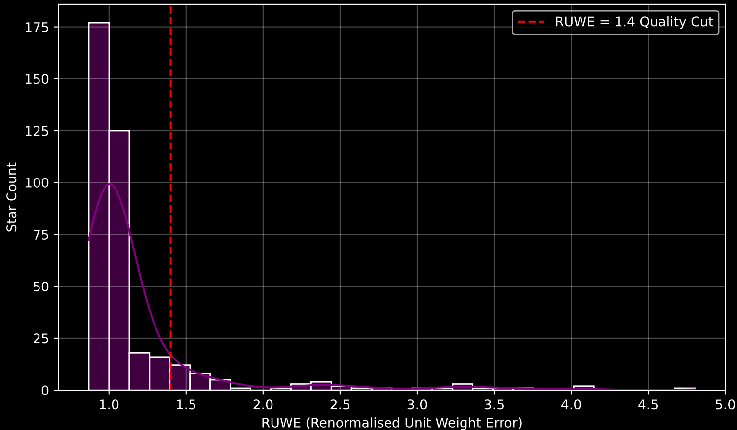
GALAH DR4 Field [6696] RUWE Distribution (n= 385)
