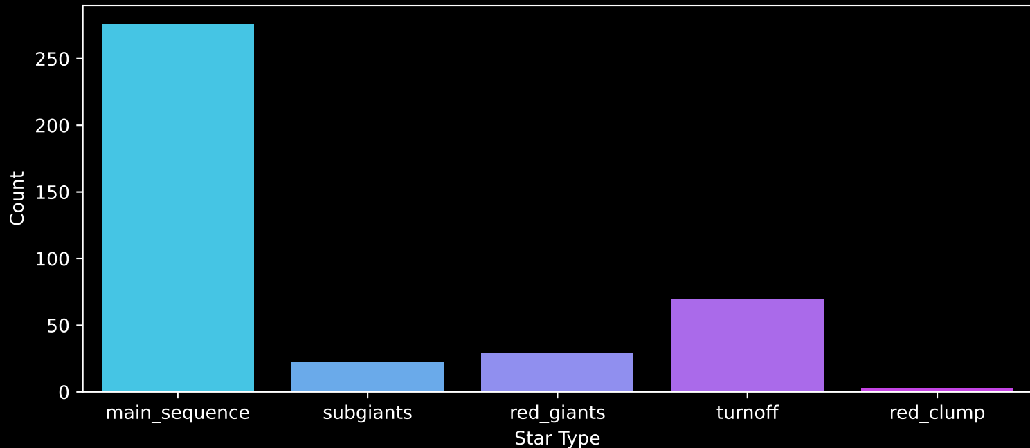
GALAH DR4 Field: [6696] Count plot of Star Type
